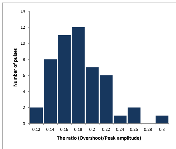
Figure 7. Overshoot to Peak amplitude ratio distribution
