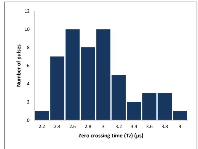
Figure 4. Zero Crossing Time ( T_z ) distribution
